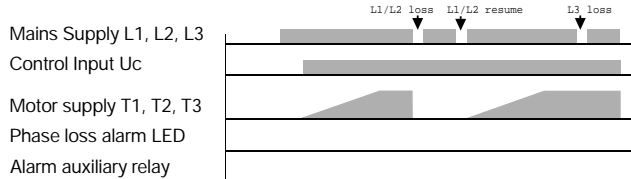
Diagram 2e: Phase loss while bypass is ON
